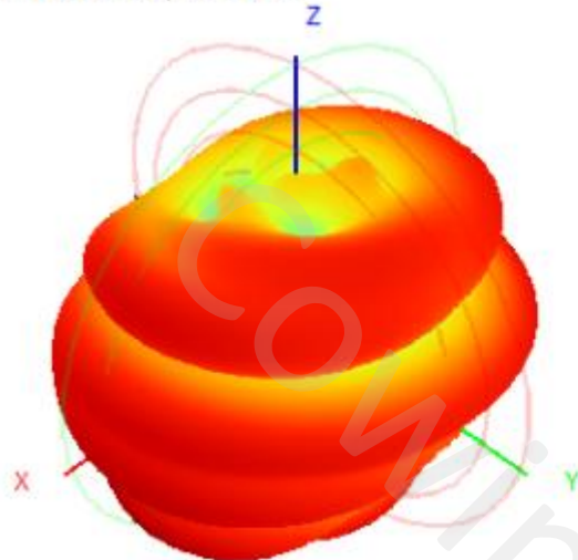
1880.0MHz H+V, Eff: 45.4%
